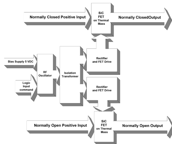
500V/5A Solid State Relay Model 3817 Form C
