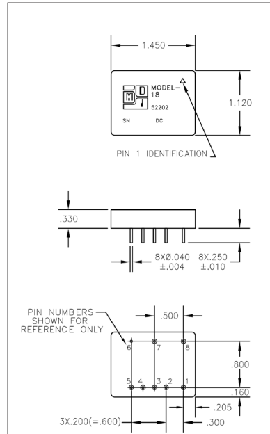
Case Style 18
