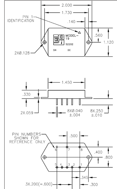
Case Style 19
