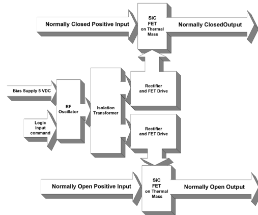
600V/10A Solid State Relay Model 53818 Form C
